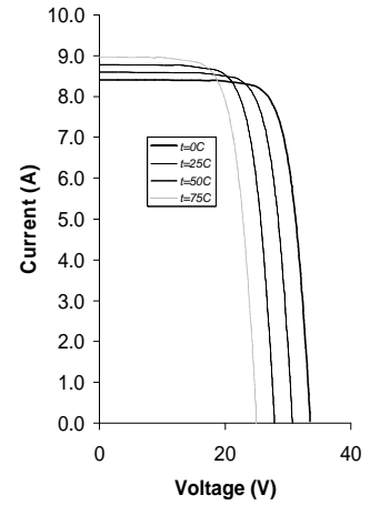
SX 3195 I-V Curves
